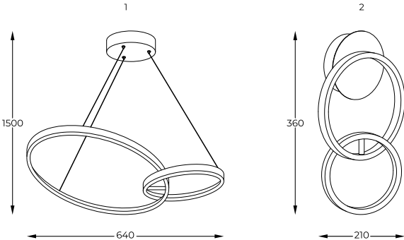
2. RANDO | Wall lamp 20002W-GD LED 18W, 900LM 3000K-4000K-6000K metal black and gold body - WALL SWITCH CCT - SETTING MEMORIZATION
