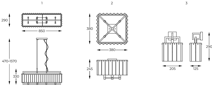
3. PALACE | Wall lamp W0523-01A-U8AC 1 x G9 MAX 42W metal matt gold body, clear bubble glass shade
