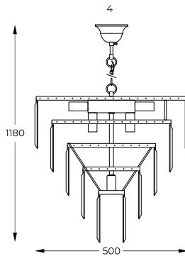
4. AMEDEO | Pendant lamp 17106/6+3+1-GD+CL 10 x E14 MAX 40W clear crystal glass gold body
