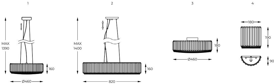
3. PRINCE | Ceiling lamp C0360-05B-F4AC 5 x G9 MAX 42W clear crystal shade, metal chrome body
