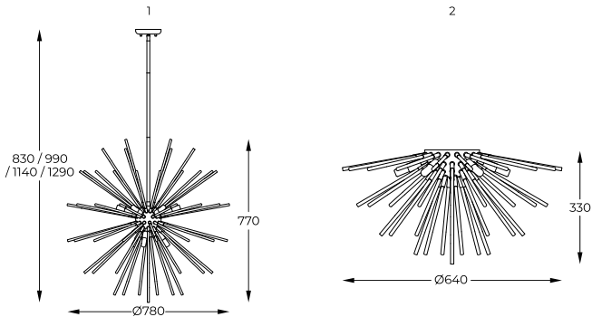
2. URCHIN | Ceiling lamp C0491-06B-F7BC 6 x G9 MAX 42W metal, french gold body black glass shade
