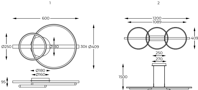
2. ALMERIA | Pendant lamp MD3913-3-3BWLT LED 35W 4100LM 3000K metal black and natural wood body plastic shade - WALL SWITCH 3-STEP DIMMING - SETTING MEMORIZATION
