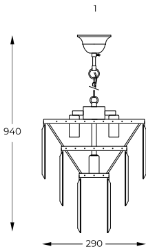
3. AMEDEO | Pendant lamp 17106/4+1-GLD 5 x E14 MAX 40W clear crystal glass gold body
