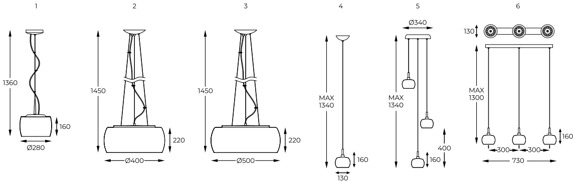
4. CRYSTAL | Pendant lamp P0076-01A-F4FZ 1 x G9 MAX 42W smoky chrome glass shade clear crystal drops inside
