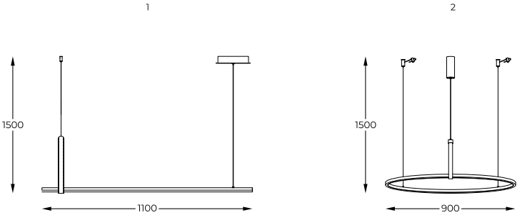
2. CLAUD | Pendant lamp 22808-WOOD LED 42W, 2000LM 3000K-4000K-6000K metal black body and veneer imitating wood - WALL SWITCH CCT - SETTING MEMORIZATION
