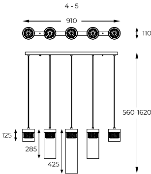
5. GEM | Pendant lamp P0389-05E-B5AC 5 x G9 MAX 28W chrome metal body, transparent crystals, transparent glass shade
