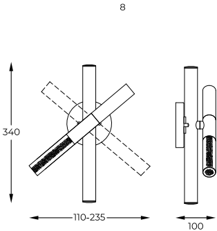
8. ONE | Wall lamp W0461-03L-P7SD 3 x LED 5W 1350LM 3000K metal matt black and french gold body, clear acrylic bar with bubbles inside
